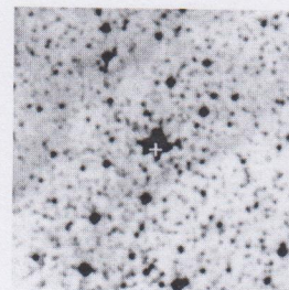
NGC 2021
